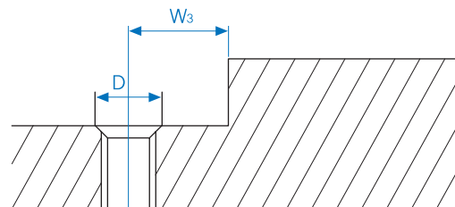
Figure 16. Dimensional tolerance between contact datum plane and mounting hole
