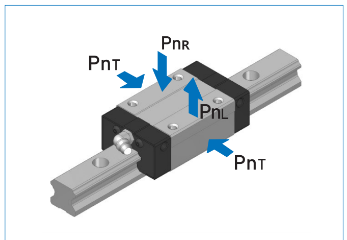
Radial Rigidity
