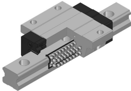
TWH-S Series (Spacer Chain Type)
