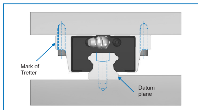
Figure 21. Linear Motion guide on the driven shaft
