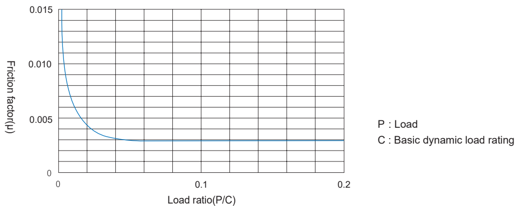
Figure 5. Relation between load ratio and friction factor
