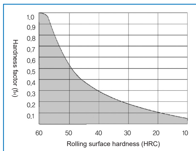
Figure 3. Hardness factor ( f_H )
