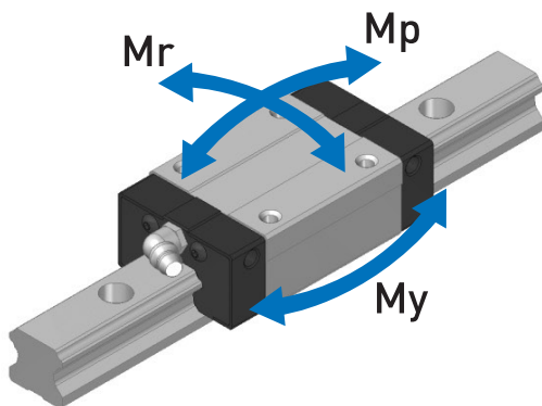
Moment Rigidity
