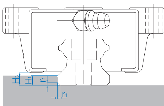
Assembly of rail datum plane
