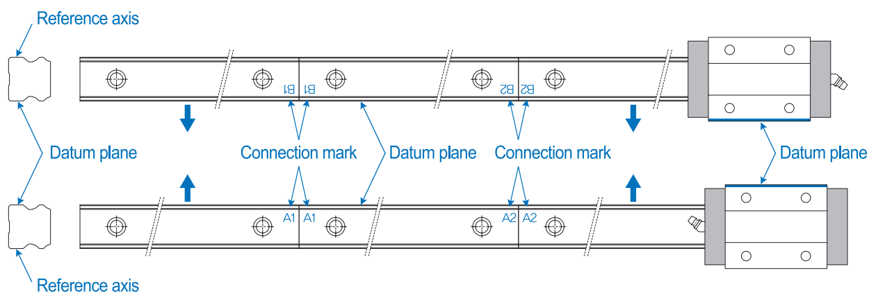
Connection of rails
