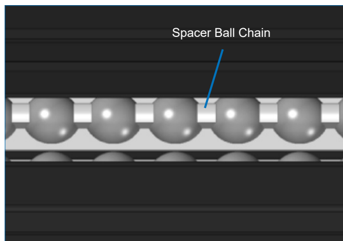
Detail of Raceway of TWH-S Series
