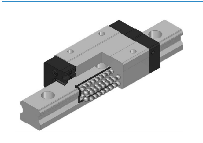
TWHS Series (Full-ball Type)
