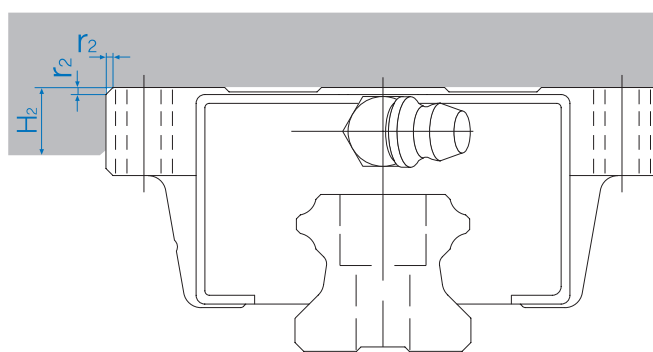
Assembly of block datum plane
