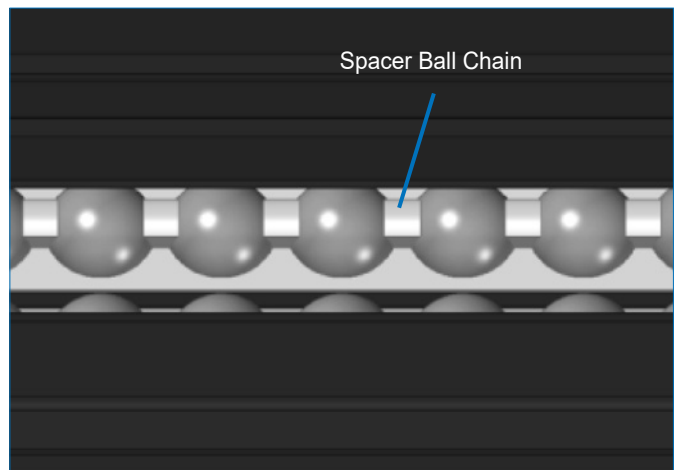
Detail of Raceway of TWHS-S Series
