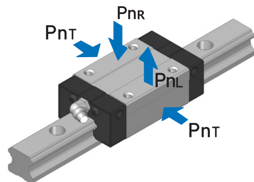
Radial Rigidity
