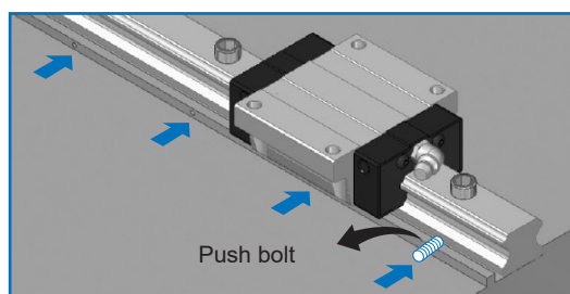
Step 4: Fasten push bolts
