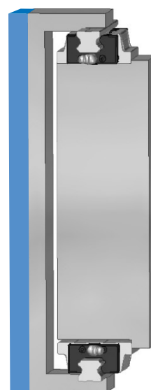
(8) Symmetrical assembly of the top and bottom of block, block transfer
